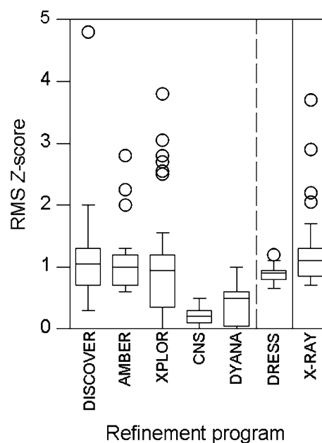
Fig. 1 RMS Z-scores for parameters describing the local geometry of protein structures refined using a selection of different programs, together with structures re-refined in explicit solvent taken from the DRESS database (Nabuurs et al. 2004). The Figure also shows Z-scores for a random selection of high-resolution (<1 Å) X-ray structures, as a comparison to what the distribution for 'high-quality' structures might be expected to look like. The RMS Z-score should be around 1: values lower than 1 indicate a narrower range of values than expected (typically indicating that restraints are too tight), while values larger than 1 indicate a wider range than expected. The local parameters measured are bond angles, bond lengths, improper dihedral angles, \omega angles and sidechain planarity. The bars indicate the range of the data (with outliers drawn as circles), and boxes indicate the quartiles and the median. Redrawn using data given in Spronk et al. (2004)
