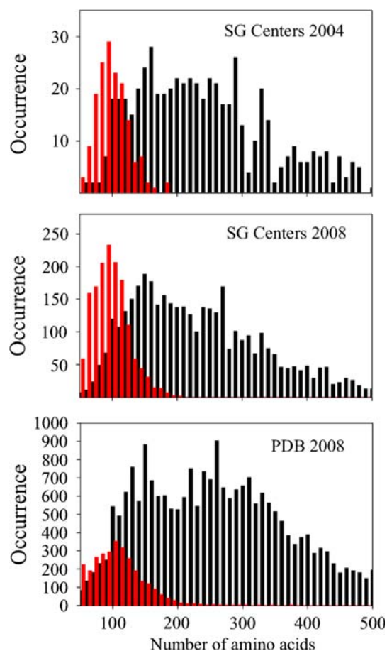
Fig. 2 Size distribution of protein structures determined by structural genomics centers and in the entire protein data bank. The top two panels show data for all structures determined by SG centers in TargetDB at 16 March 2004 (top) and 14 September 2008 (middle), taken from the TargetDB database http://targetdb.pdb.org/ (Chen et al. 2004). The bottom panel shows data for the entire PDB from January 2004 to November 2008, and is thus roughly comparable in time to the middle panel. Note the small but significant number of structures with >200 residues in the bottom panel. There was no attempt to remove duplicates and close duplicates. Data on proteins of less than 50 residues in length are not shown. Crystal structures are shown in black and NMR structures in red
